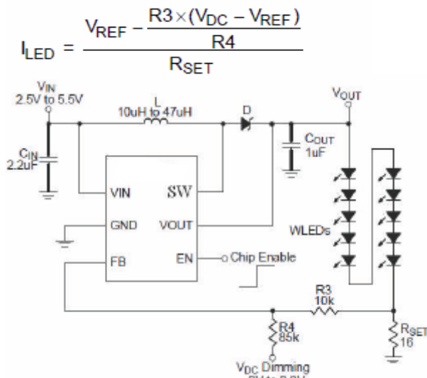
Figure 4 Dimming Control Using a DC Voltage
