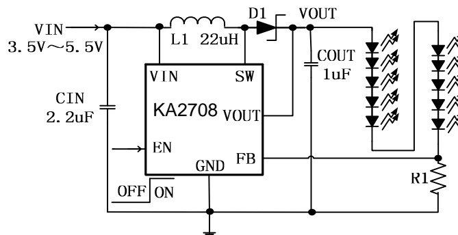
Figure 1. Basic Application Circuit with KA2708
