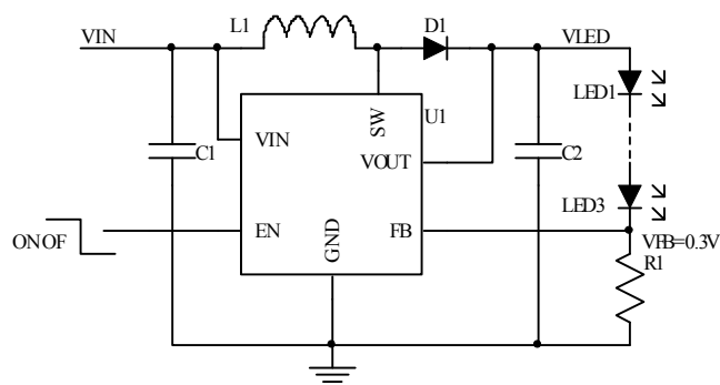
Figure 10 High-light LED Flash
