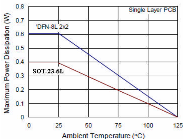
Figure 7 Derating Curves for KA2708 Packages
