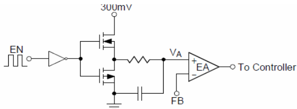
Figure 3 Block Diagram of Programmable FB Voltage Using PWM Signal
