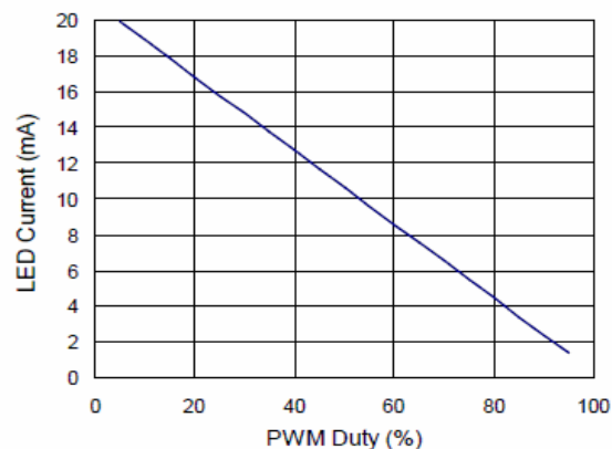
Figure 6 PWM Duty Cycle vs LED Current
