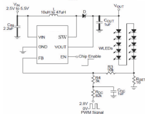
Figure 5 Dimming Control Using a Filtered PWM Signal
