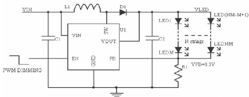
Figure 8 LED Backlighting
